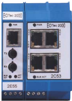
2E55 Switched Media converter with a 2C53 Ethernet Switch
